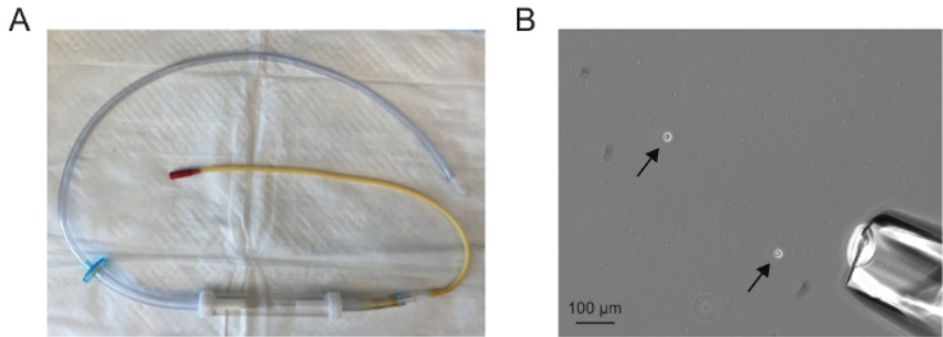
Figure 1. Single cell isolation. (A) An assembled microaspirator. (B) A 10X field showing dissociated cells (arrows) and microaspirator needle (lower right corner). Aspirating single cells is easiest when there are between one and five cells in a 10X field. Please click here to view a larger version of this figure.
