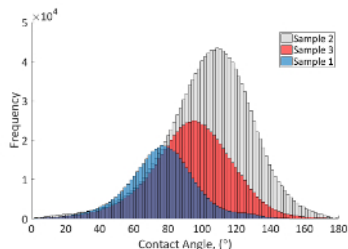
Figure 6: Distributions of the contact angle measurement of the three mini-samples. Sample 1 has a mean contact angle of 77^\circ \pm 21^\circ with 462,000 values shown in blue. Sample 2 has a mean contact angle of 104^\circ \pm 26^\circ with 1.41 million values shown in gray. Sample 3 has a mean contact angle of 94^\circ \pm 24^\circ with 769,000 values shown in red. Please click here to view a larger version of this figure.
