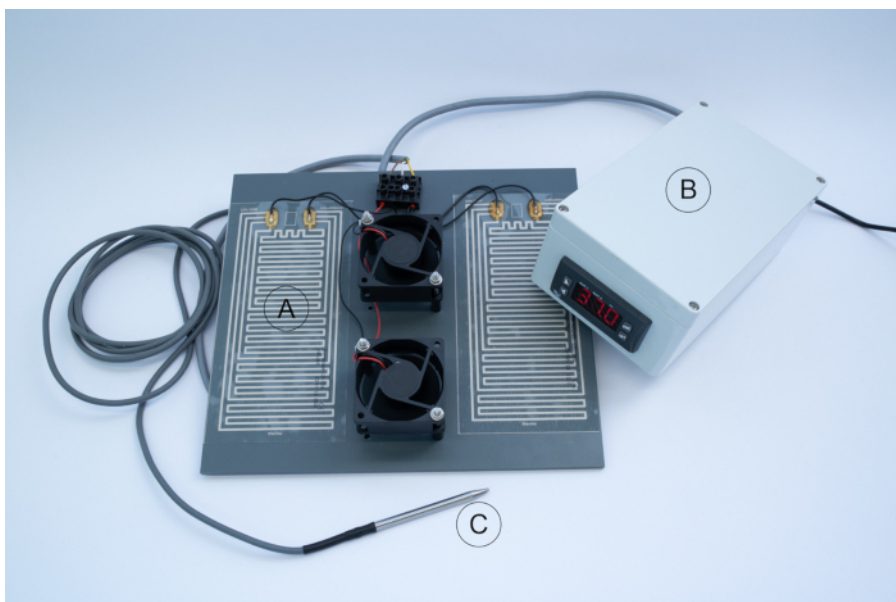
Figure 8: Complete field incubator electrical core. Heating unit (A), control unit (B) and temperature probe (C). Please click here to view a larger version of this figure.
