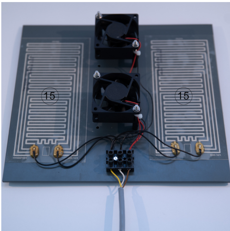
Figure 7: Cable connection of heating foils 15 with PID temperature controller. Please click here to view a larger version of this figure.
