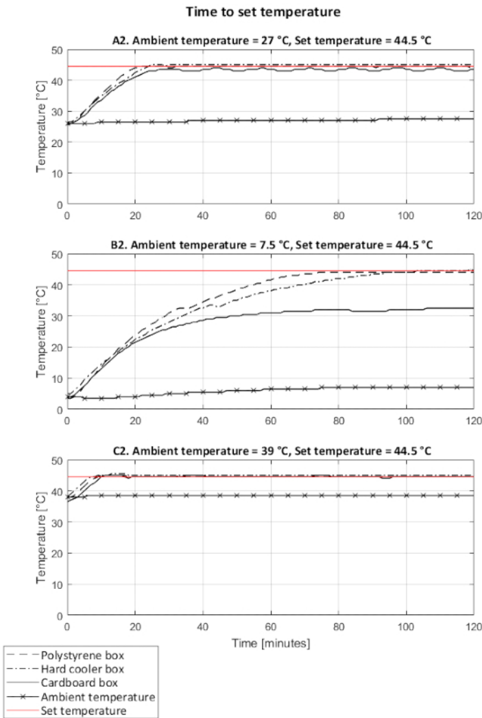
Figure 12: Time to reach set temperature (44.5 °C) of the incubator set-ups under different ambient temperature conditions. Performances of incubators with a shell made of a polystyrene foam box, a hard cooler box, and a cardboard box covered with a survival blanket. At room ambient temperature (a), cold ambient temperature (b), and warm ambient temperature (c). Temperatures recorded on the support rack of the incubators. Please click here to view a larger version of this figure.
