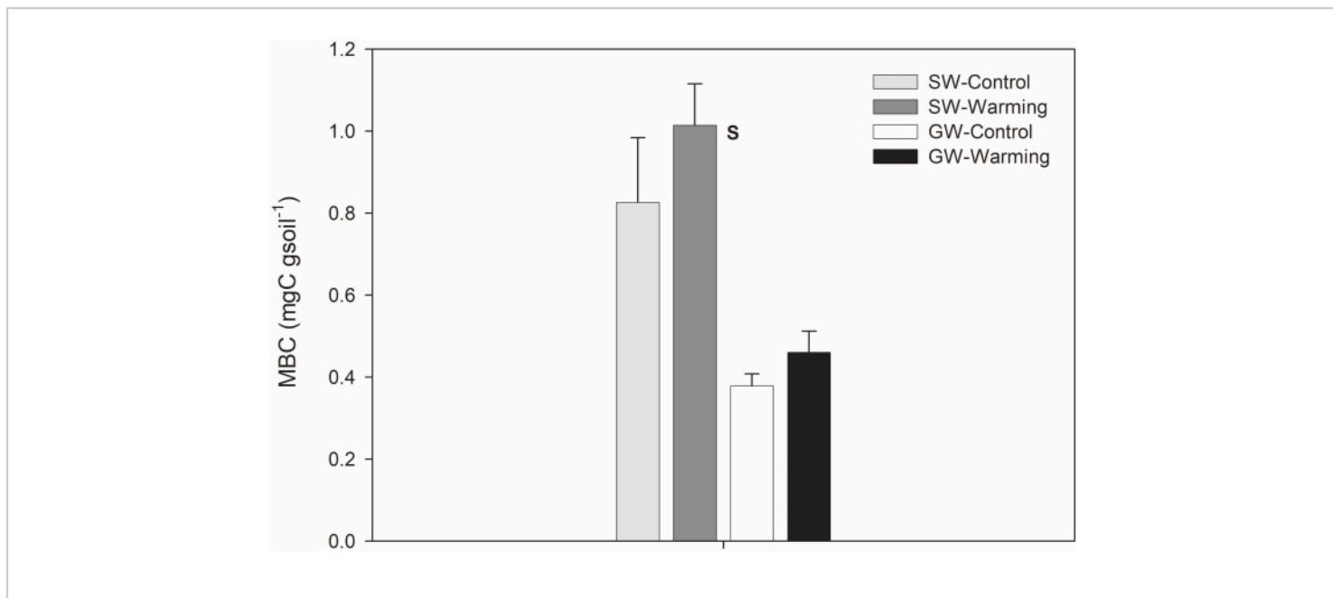
Figure 4: Mean ( \pm SE) MBC under control and warming treatments in SW and GW in a 42-day soil incubation experiment. MBC = microbial biomass carbon; N = 4 in each collection. S denotes significant effect of warming scenario (SW vs. GW), at p < 0.05 , based on a three-way repeated measures ANOVA. Please click here to view a larger version of this figure.
