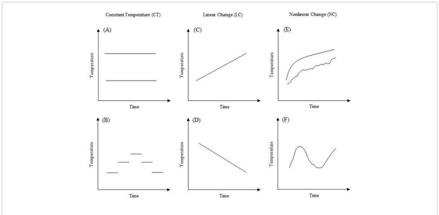
Figure 1: The illustration of temperature change mode in a soil warming experiment as conceptualized from Table 1. (A) Constant temperature (CT) adopted by most studies. (B) Constant temperature with varying magnitude (CT v ). (C,D) Linear change (LC) with positive and negative rates. (E,F) Nonlinear change (NC) with irregular pattern and diurnal pattern.
