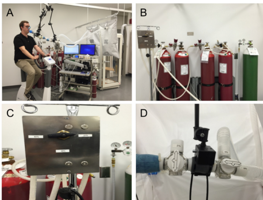
Figure 1: Multiple F I O 2 DL CO Setup. (A) Setup overview. (B) Compressed-gas cylinders containing 21%, 40%, and 60% O 2 with 0.3% CO, 0.3% methane, and balance nitrogen, as well as a supplemental oxygen compressed-gas cylinder. (C) Three-way valve selector for the three F I O 2 DL CO tanks. (D) Valve switch for three-way valves in the series for the selection of F I O 2 for pre-breathing. Please click here to view a larger version of this figure.
