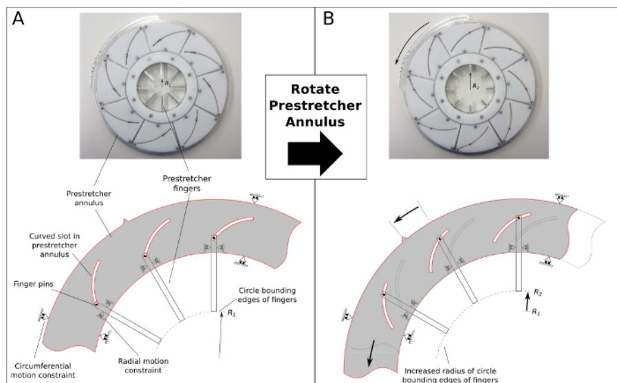
Figure 5. Operating principle of the membrane prestretcher. (A) Several metal fingers are attached to a plastic annulus and are constrained to move in a linear (radial) fashion along their length. The annulus is constrained to move circumferentially. The plastic annulus has several curved slots machined into it, into which the metal pins of the fingers reside. Radius of a circle bounding the edge of the fingers is R_1 . (B) The prestretcher annulus is rotated counter-clockwise, the fingers translate simultaneously, increasing the radius of the circle bounding the finger edges from R_1 to R_2 . Please click here to view a larger version of this figure.
