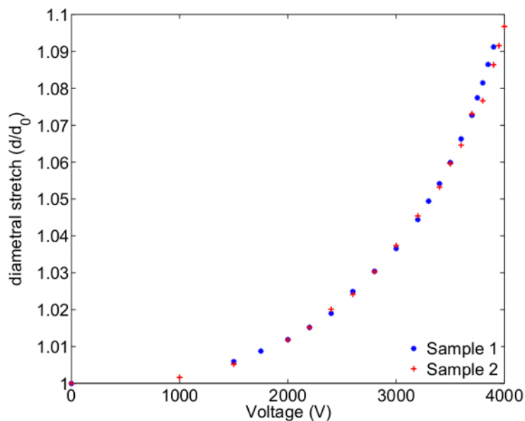
Figure 8. Actuation of the demonstrator. Outside diametral stretch as a function of the applied voltage for two devices with a thickness (after prestretch) of 34.5 \mu\text{m} . An increase of diameter of about 10% is observed at the maximal applied voltage. Please click here to view a larger version of this figure.
