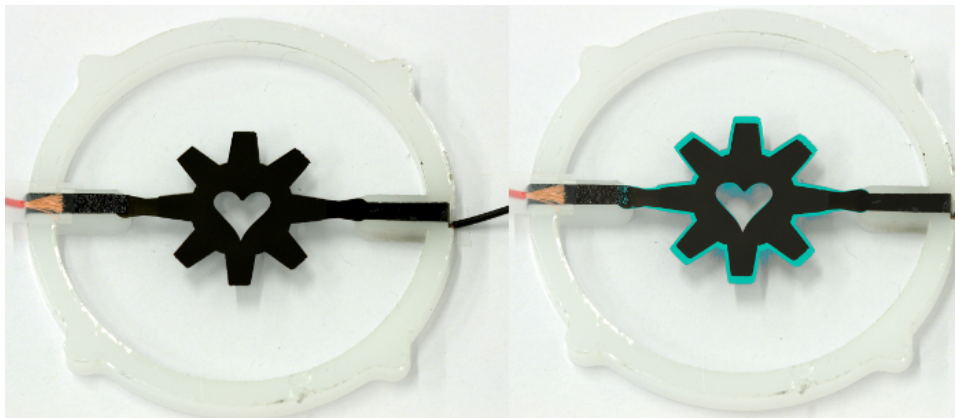
Figure 2. Demonstrator actuator fabricated in this protocol. Left: finished device comprising a stretched silicone membrane fixed on a frame, a pair of compliant electrode patterned on both sides of the membrane, and electrical connections. Right: composite picture showing the rest state (black) and activated state (cyan). A 10% increase in the diameter of the structure is observed with 4 kV applied across the electrodes. Please click here to view a larger version of this figure.
