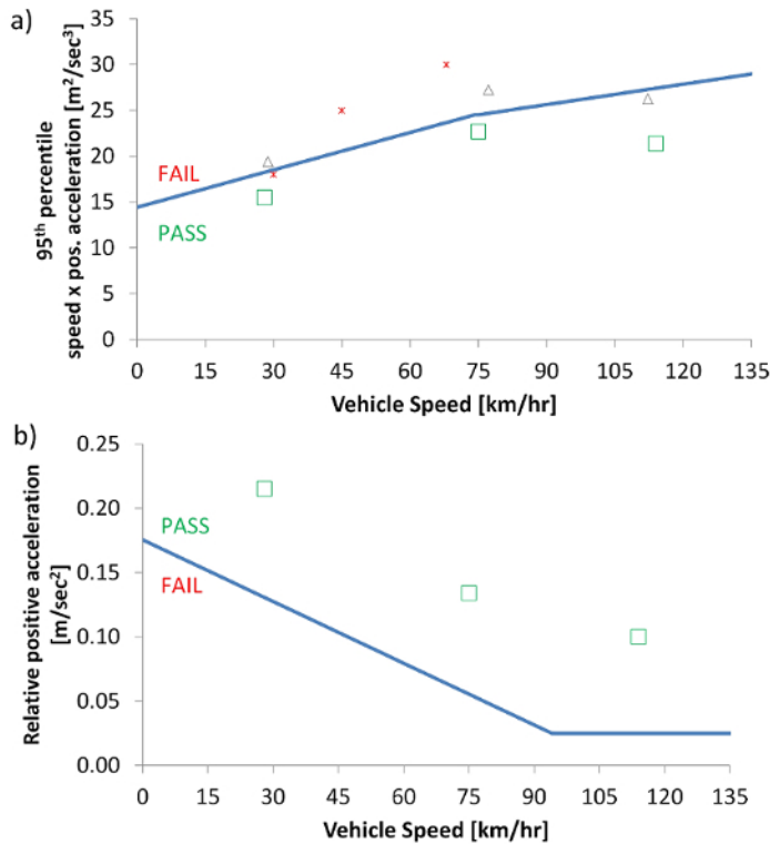
Figure 4: Indices to check the excess or absence of driving dynamics. (a) 95 th percentile of the product of instantaneous speed and positive acceleration during urban, rural, and motorway driving. (b) Relative positive acceleration during urban, rural, and motorway driving. The open squares are the experimental results. The open triangles are results with aggressive driving in the same car. The asterisks are aggressive trips in German cities. The continuous line shows the permitted limits. The pass or fail areas are also shown. Please click here to view a larger version of this figure.
