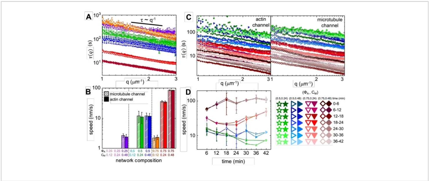
Figure 4. Time-resolved differential dynamic microscopy (DDM) measures the rate and type of motion of actin and microtubules in active composites. (A) DDM is performed on microtubule (top, open symbols) and actin (bottom, filled symbols) channels of time-series to determine characteristic decay times \tau vs wavenumber q for both actin (filled symbols) and microtubules (open symbols) as described previously 17,26 . All curves follow \tau \sim q^{-1} scaling, indicating ballistic motion, with speeds v that are determined via fits to \tau(q) = (vq)^{-1} . Faster speeds correspond to smaller \tau(q) values for any given q . Symbol colors and shapes correspond to (\Phi_A, c_M) combinations shown in B. (B) Contraction speeds v are determined via fits to \tau(q) curves shown in A, which are averaged over all lag-times for the duration of each 45 min time-series. (C) Time-resolved DDM (trDDM) quantifies how the dynamics vary over time by evaluating \tau(q) for actin (filled symbols, left) and microtubules (open symbols, right) for consecutive 6 min intervals (denoted by different shades of the same color) during the 45 min activation time. trDDM is performed for each (\Phi_A, c_M) combination (denoted by different symbols and colors) as described in the legend in lower right. \tau(q) curves shown in C follow similar scaling and trends as those in A but also show time-dependence for certain (\Phi_A, c_M) compositions, most notably for \Phi_A = 0.75 . (D) Contraction speeds for actin filaments (closed symbols) and microtubules (open symbols) are determined from fits to corresponding \tau(q) curves. Error bars in all plots represent the standard error of values across three to five replicates. This figure has been modified from reference 17 .
